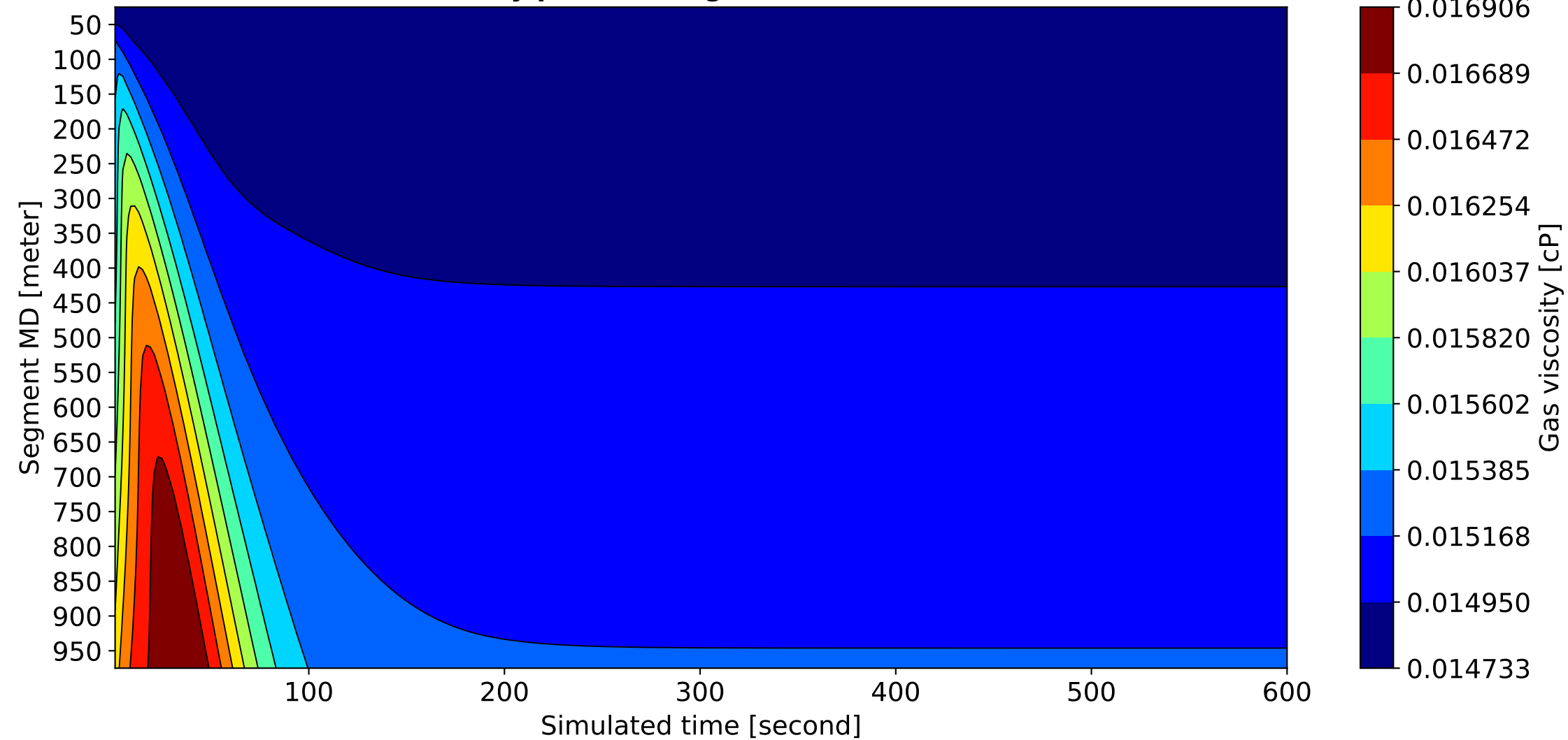
Gas viscosity profile along the wellbore over time
